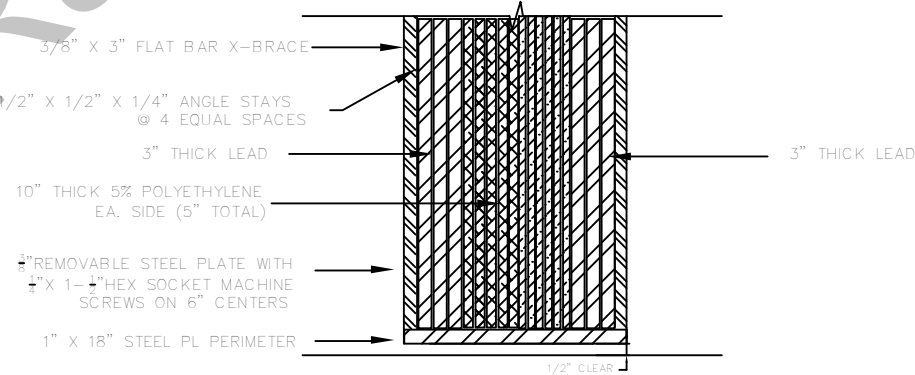
SILL DETAIL DOOR SECTION ① SCALE NTS
